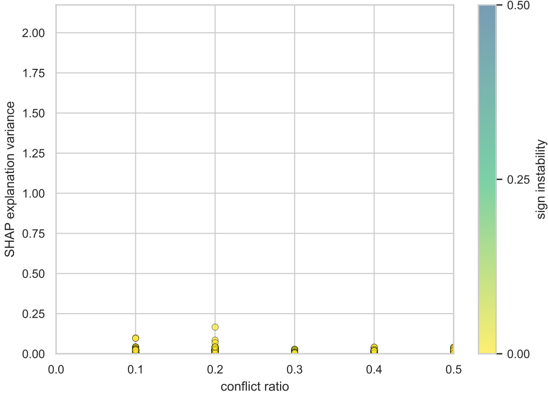
cat__flag_S0: SHAP explanation variance (Spearman r = -0.077)
